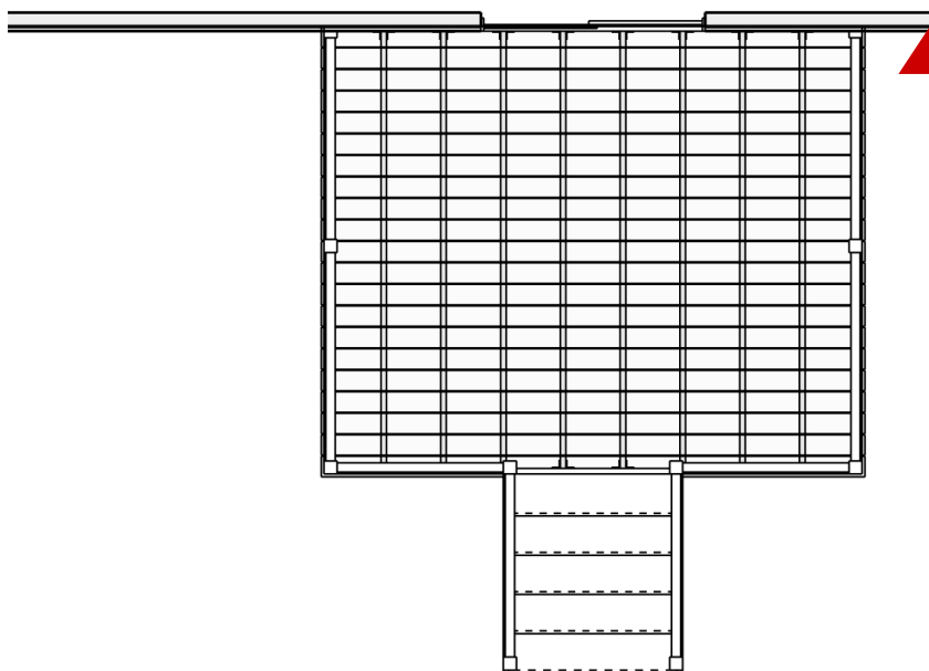
PROPOSED MAIN FLOOR LAYOUT
