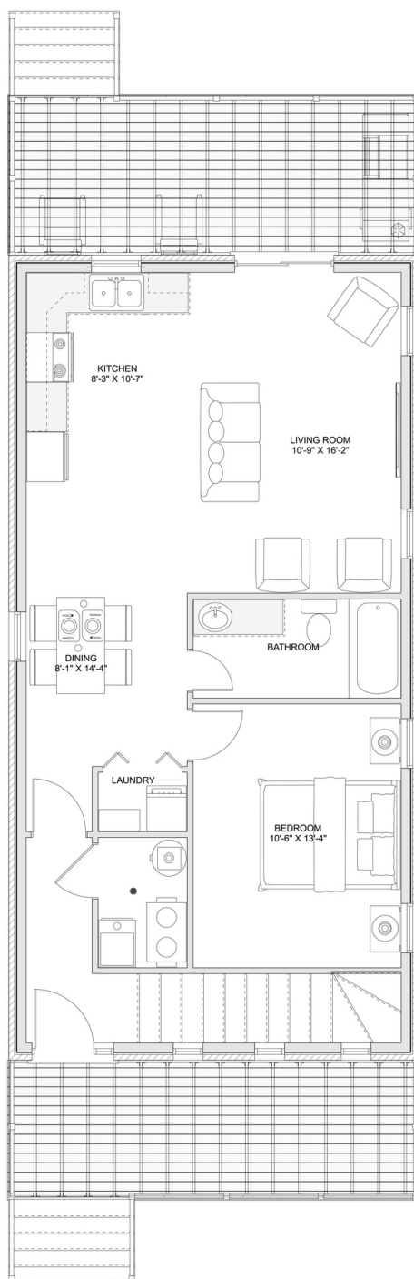
MAIN FLOOR
