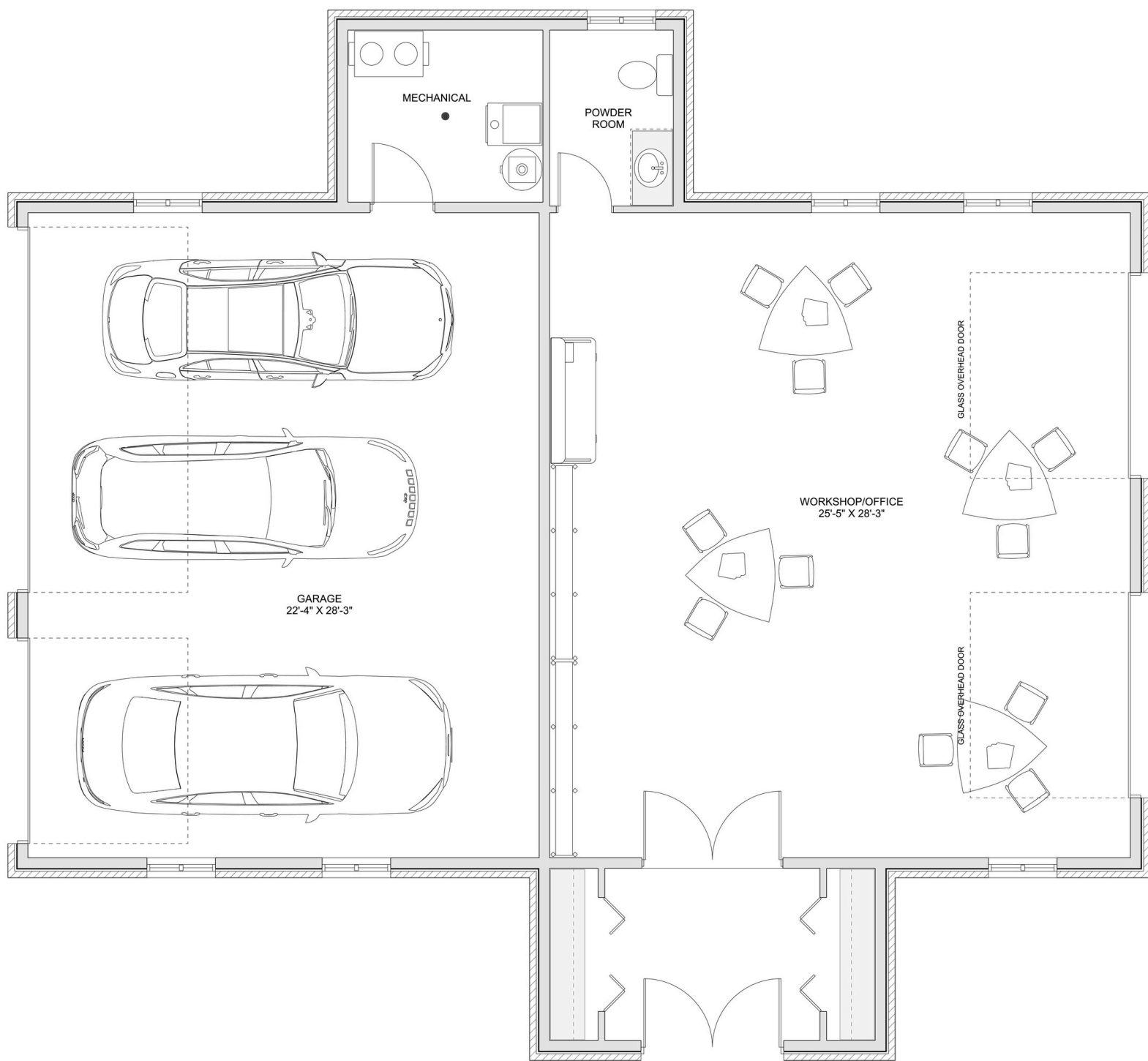
MAIN FLOOR
