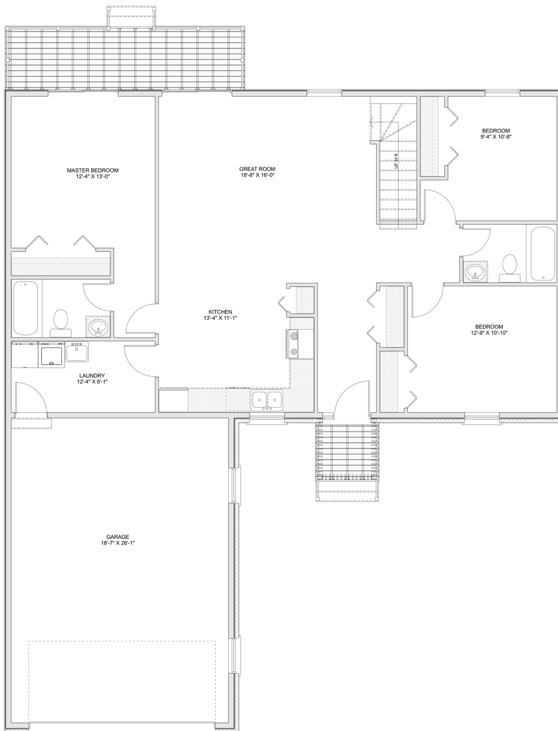
MAIN FLOOR
